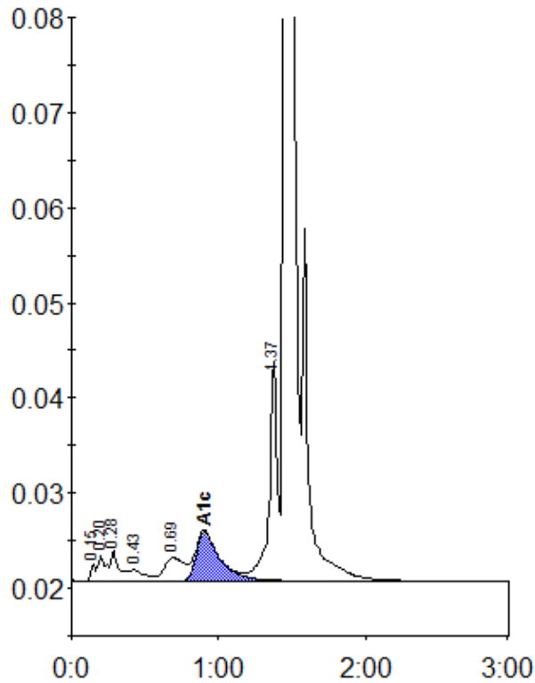
Peak table - ID: 10401254
